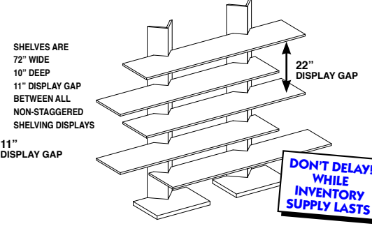
72" WIDE STAGGERED DISPLAY SHELF
