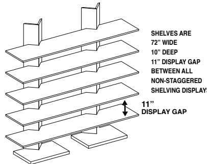
72" WIDE STRAIGHT DISPLAY SHELF
